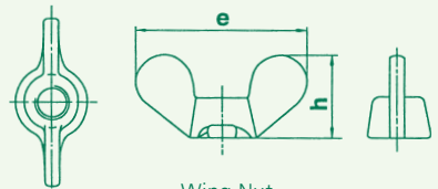
Wing Nut
